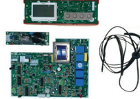
220596 KIT MAIN BOARD, IGNITION & T/STAT 2008 (4721216SP)
